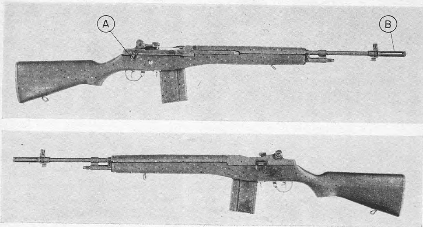
The new U. S. Army Rifle M14, known as the T44 during development, it fires the 7.62 mm. NATO cartridge, and weighs 8.7 lbs. unloaded against 9.6 lbs. for the M1 (Garand) rifle. Balance and handling qualities are excellent. Magazine capacity is 20 rounds instead of 8 in the M1. A change lever (A) gives choice between semi- and full-automatic fire. Under current plans the regularly issued rifles will be equipped for semi-automatic fire only. Barrel length is 22". The slotted flash hider (B) resulted from fundamental investigations which revealed that flash is best suppressed by extending rods before the muzzle to break up the compression wave of the emerging gas.
