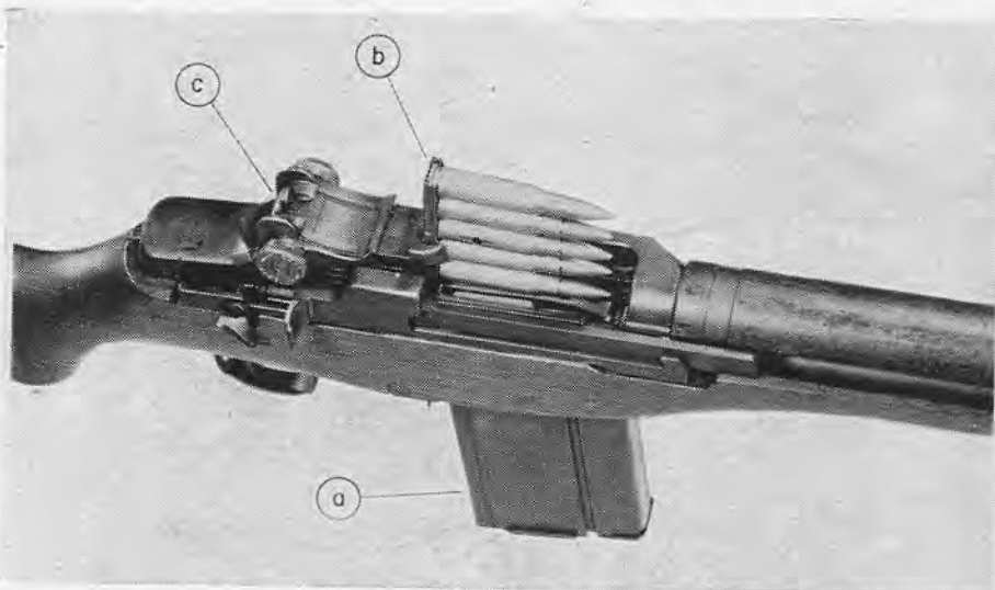
The magazine (a) of the M14 can be loaded from clips (b) when in the rifle. It is a detachable box, a supply of which can be carried loaded. Aperture rear sight (c) is provided with strong 1-minute clicks in both elevation and windage, as in M1 rifle
